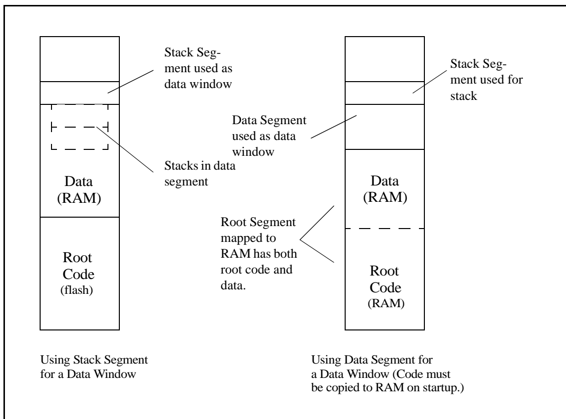
Figure 3-6. Schemes for Data Memory Windows
